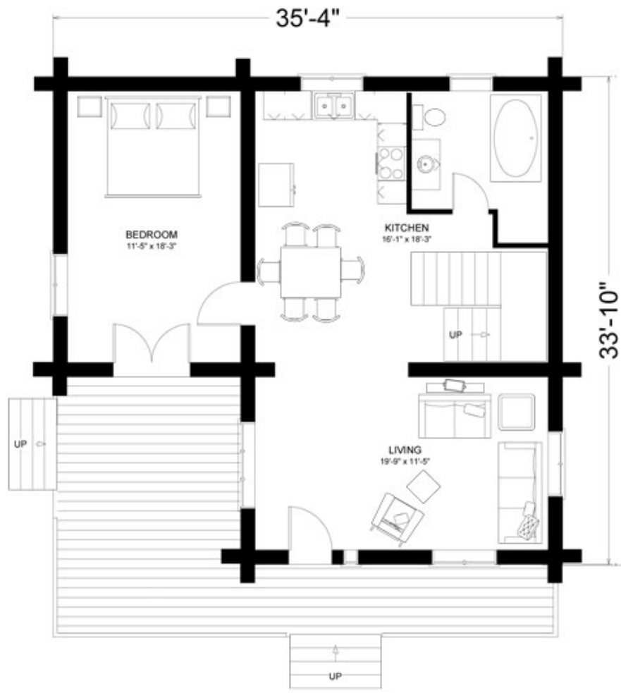
MAIN FLOOR 1065 SQ FT
