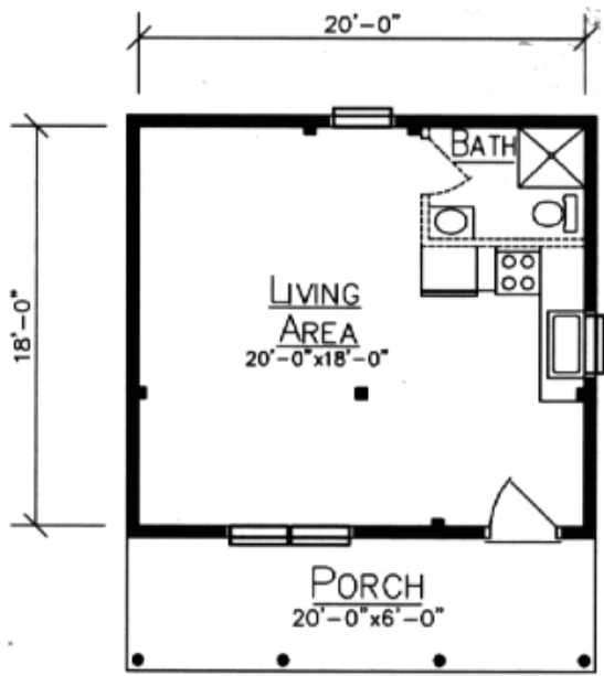
MATAGAMON FIRST FLOOR PLAN
