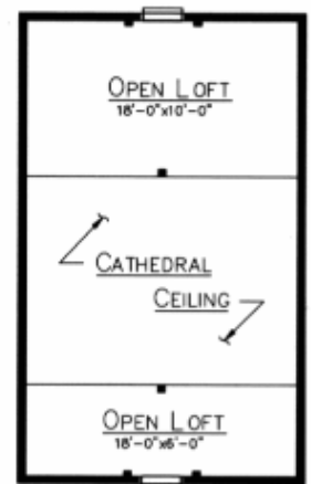
BASKAHEGAN LOFT PLAN
