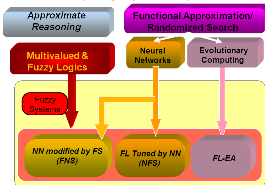
Figure 85: Hybrid Fuzzy Logic Systems (adapted from http://www-bisc.cs.berkeley.edu )
