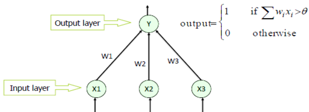
Figure 67: The perceptron (adapted from http://www.saedsayad.com/artificial_neural_network_bkp.htm )
