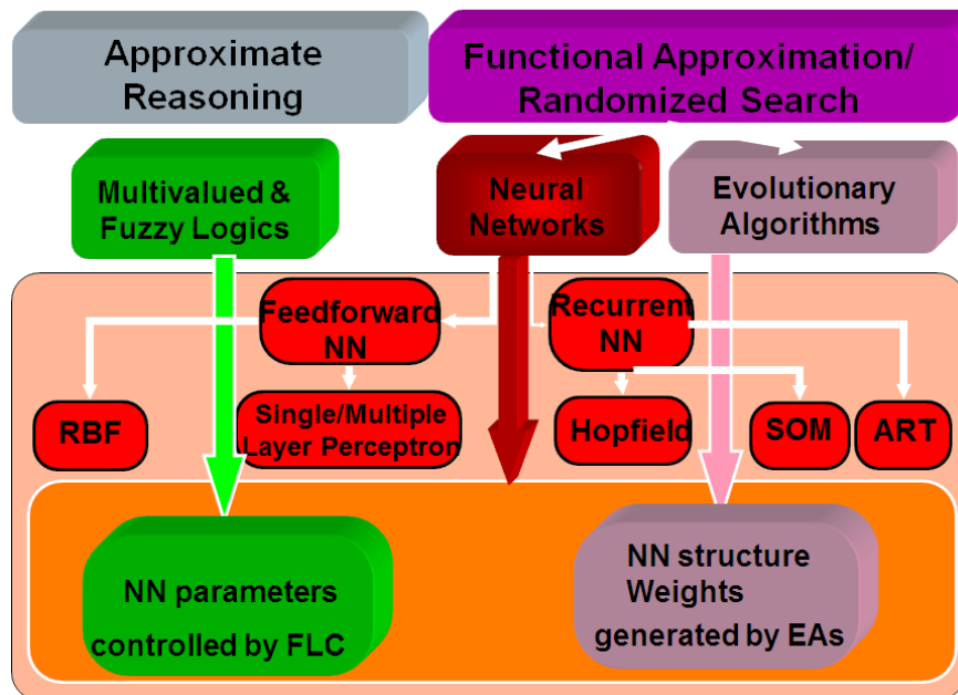
Figure 86: Hybrid Neural Network Systems (adapted from http://www-bisc.cs.berkeley.edu )
