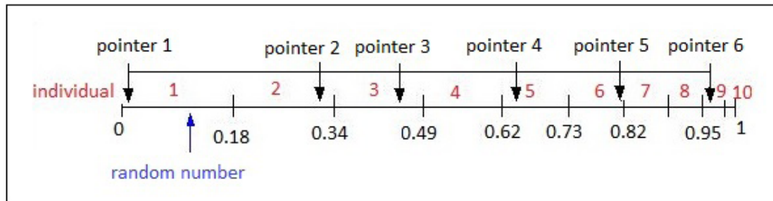
Figure 38: Stochastic universal sampling (adapted from http://www.geatbx.com/ )
