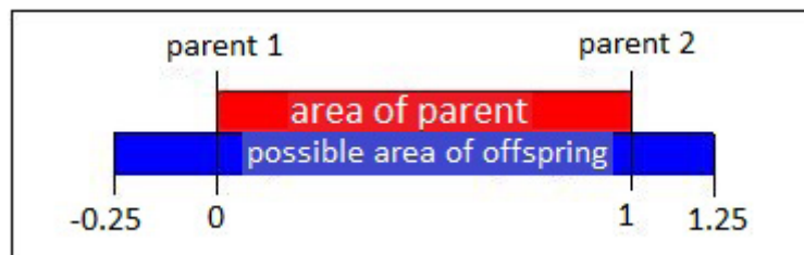
Figure 43: Area for variable value of offspring compared to parents in intermediate recombination (adapted from http://www.geatbx.com/ )
