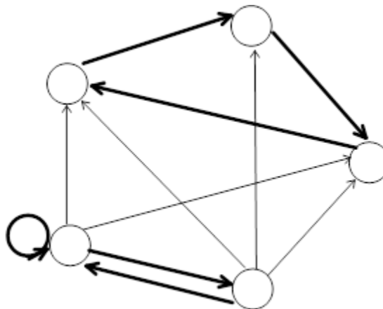
Figure 66: Recurrent networks
