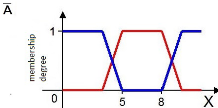
Figure 7: Fuzzy Complement
