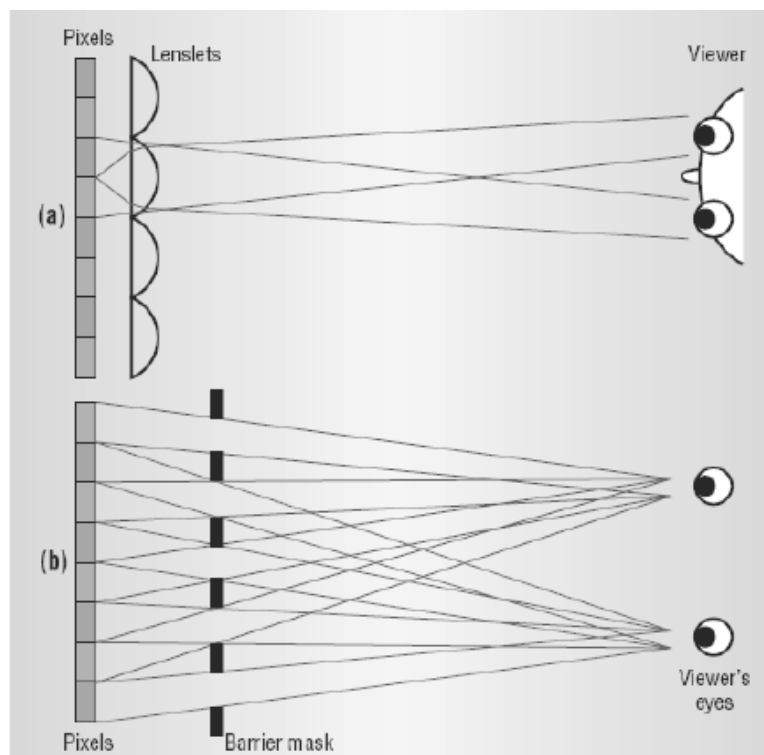
Figure 5.10: Auto-stereoscope arrangements
