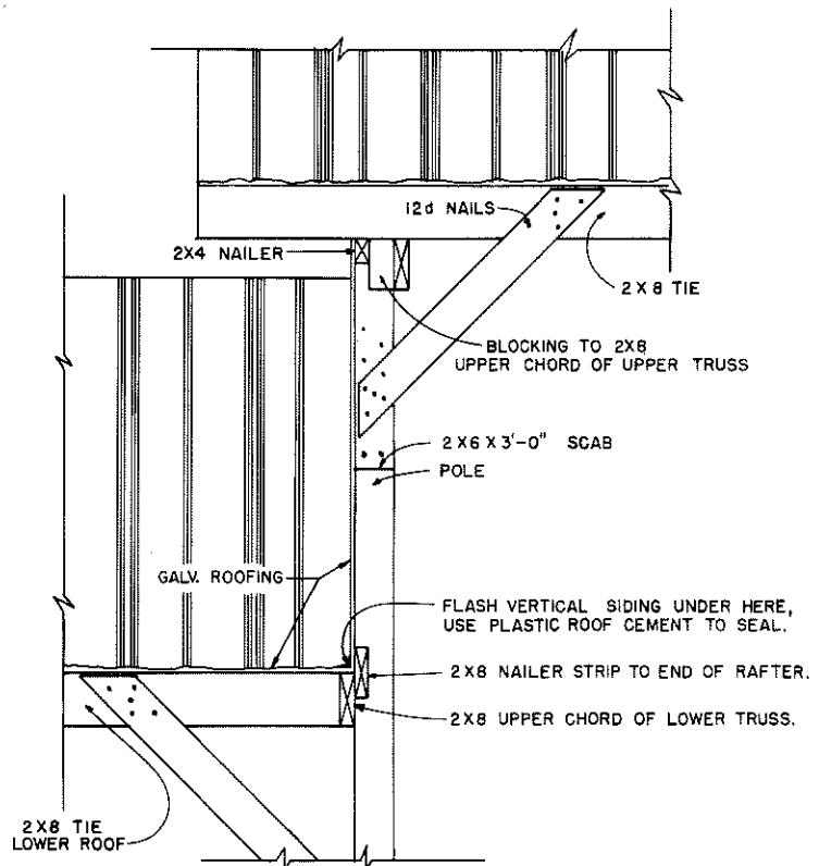
DETAIL A SCALE: 3/4" = 1'-0" 12" 6" 0"
