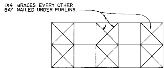
ROOF BRACING SYSTEM NOT TO SCALE
