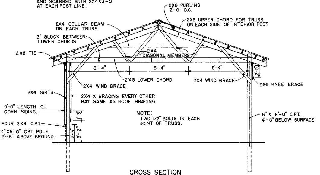
CROSS SECTION
