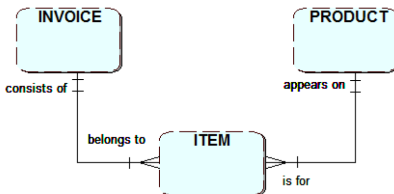
Resolved M:N
