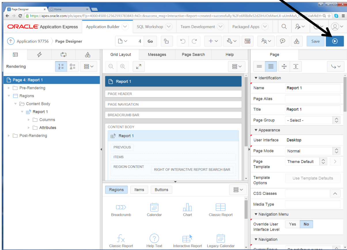
Page Designer
