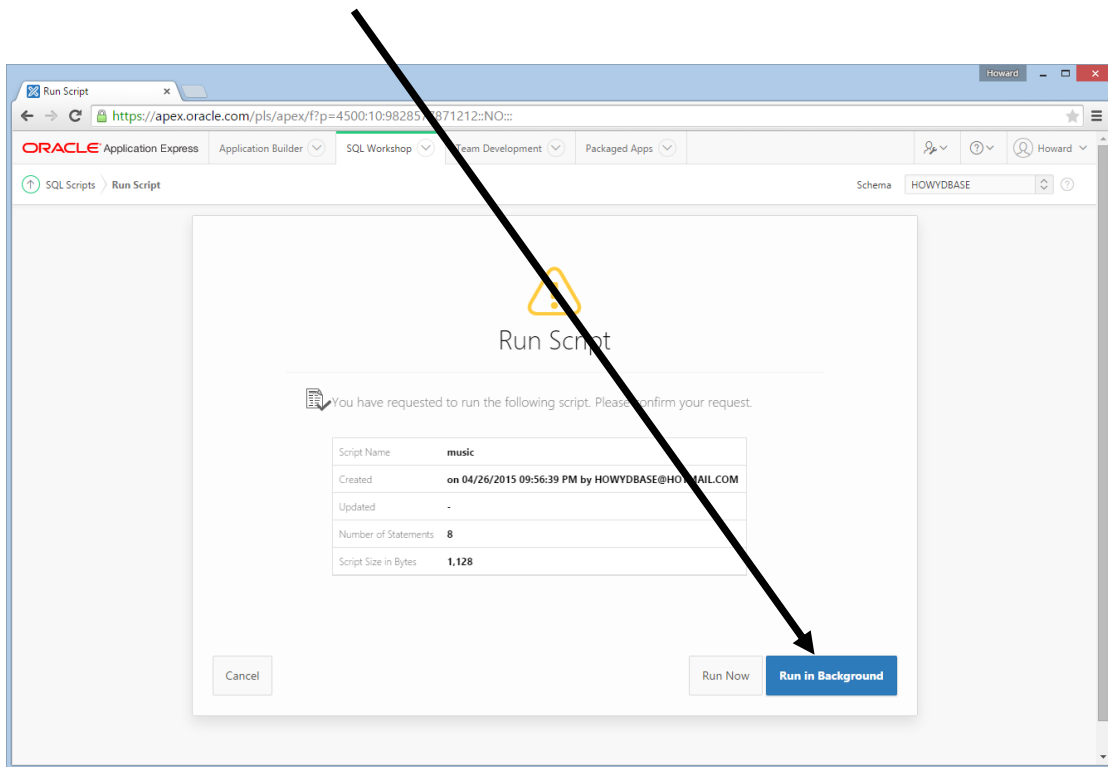
Run Script
