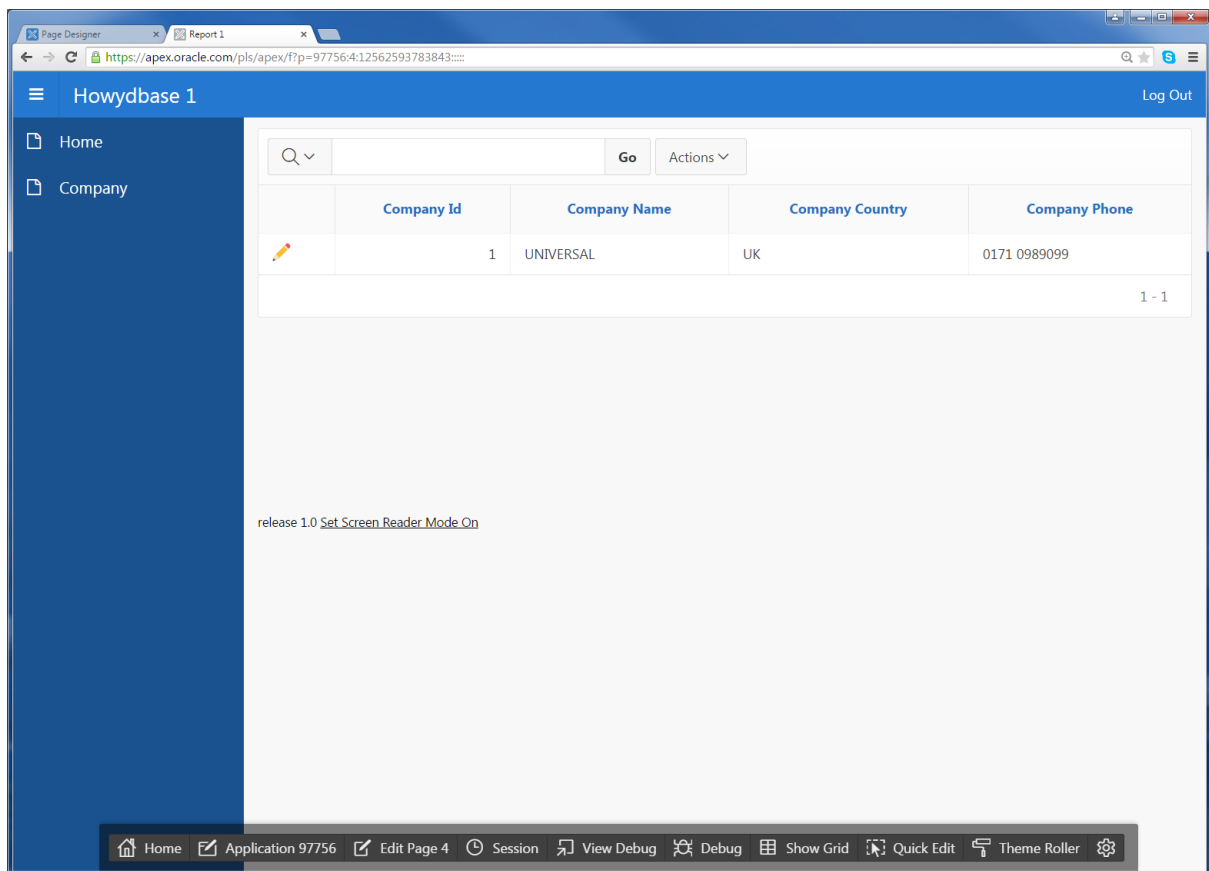
Company Page
