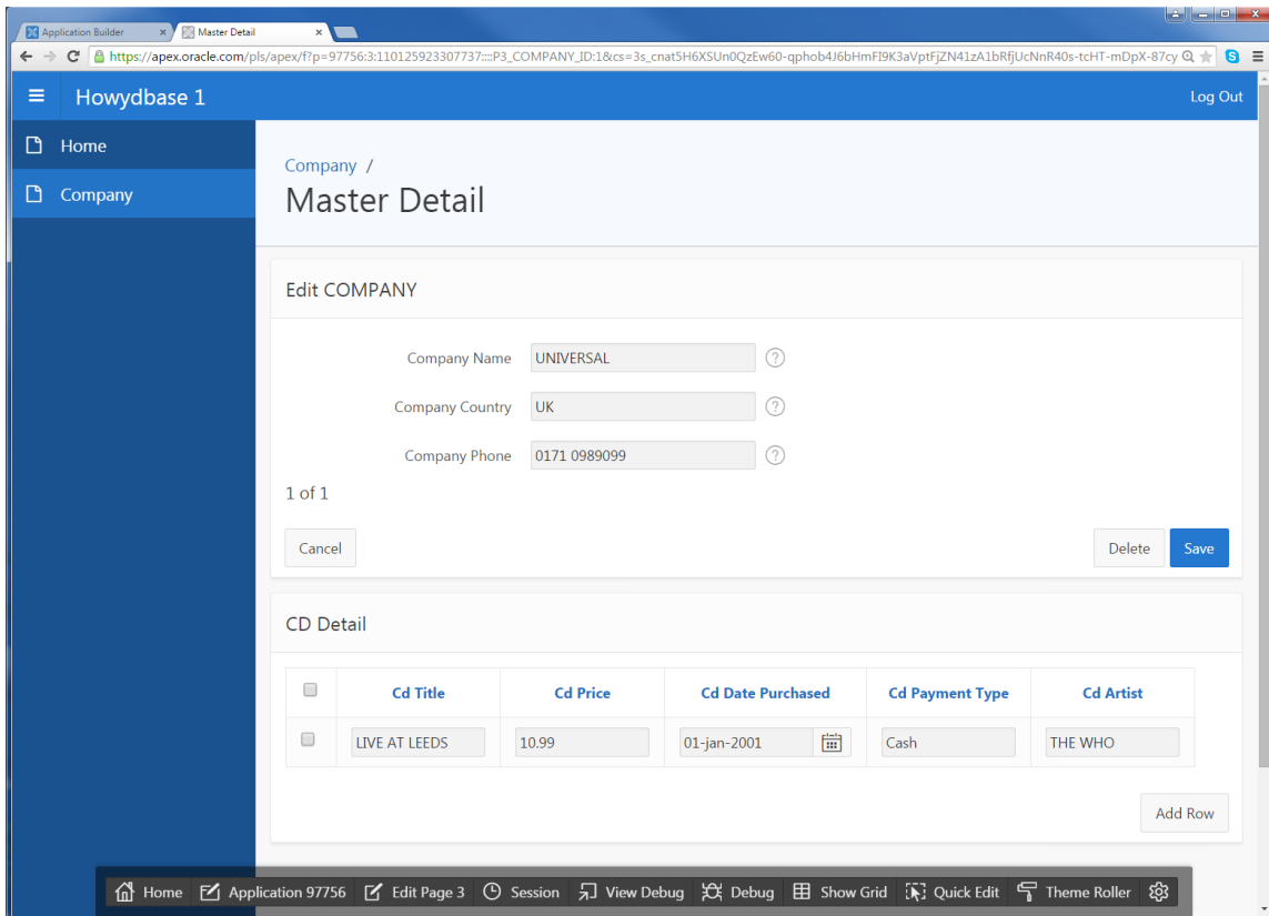
Detail Row
