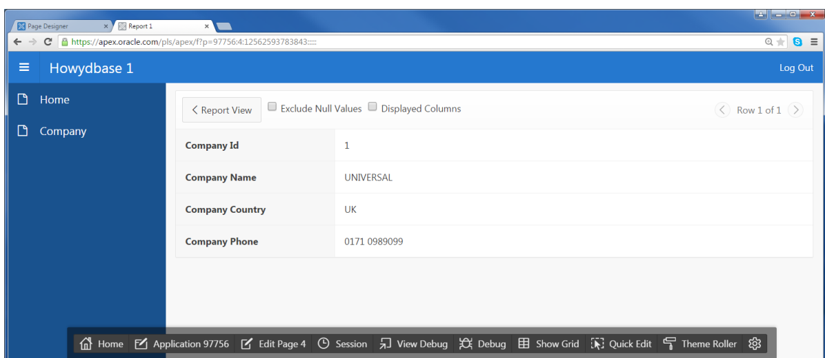
Report View
