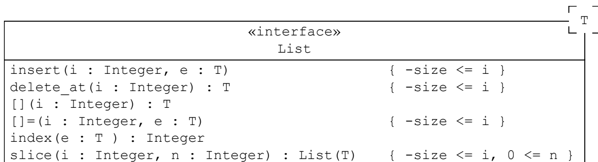
Figure 1: The List Interface
