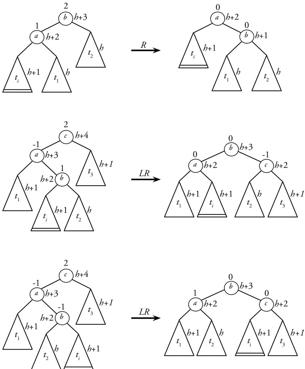
Figure 2: Balance Factor 2 Rotations
