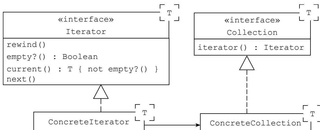
Figure 1: The Design Iterator Pattern
