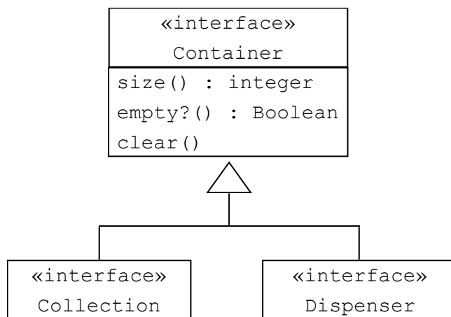
Figure 2: Top of the Container Taxonomy
