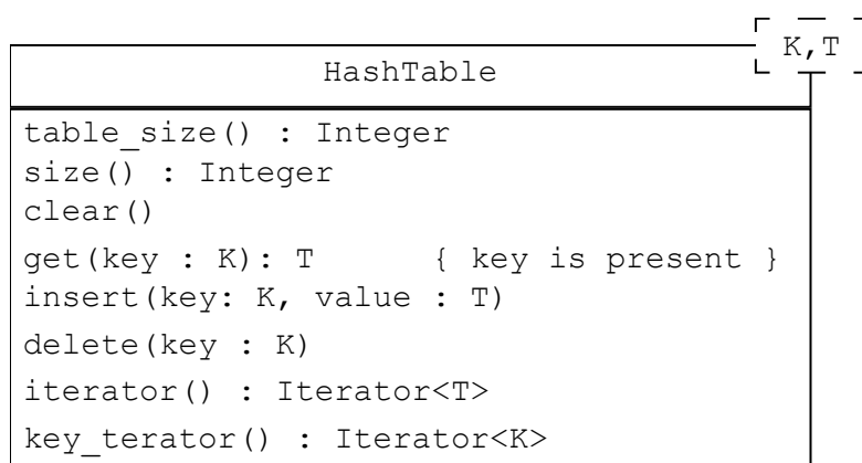
Figure 1: A HashTable Class
