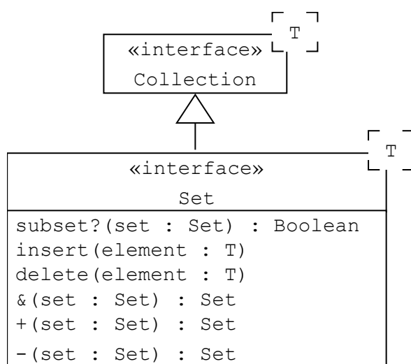
Figure 1: The Set Interface
