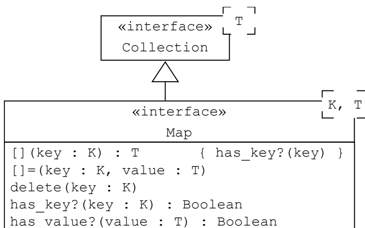
Figure 1: The Map Interface
