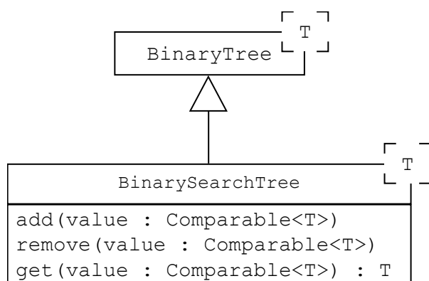
Figure 4: The BinarySearchTree Class
