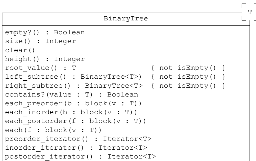
Figure 2: The BinaryTree Class
