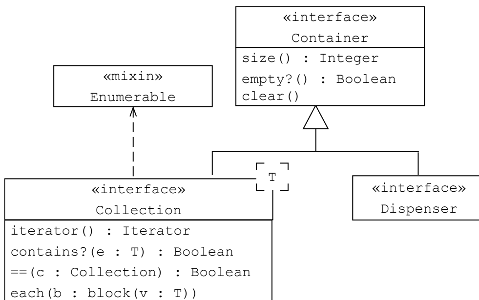
Figure 3: The Collection Interface in the Container Hierarchy
