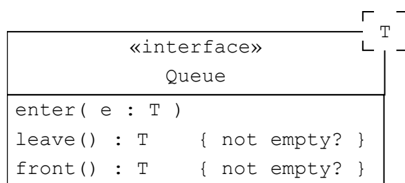
Figure 1: The Queue Interface
