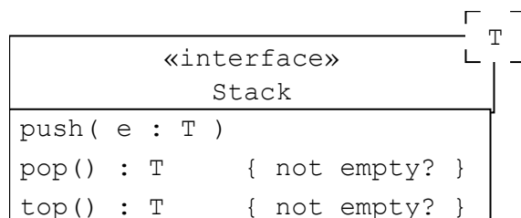
Figure 1: The Stack Interface
