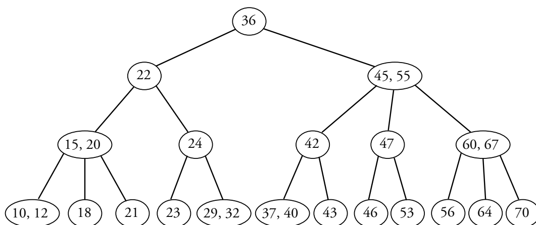
Figure 1: A 2-3 Tree
