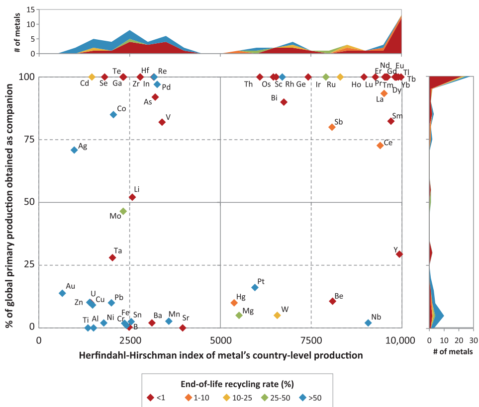
Fig. 4. Companionship, primary production concentration, and end-of-life recycling for 62 metals. Primary production concentration is measured by the HHI, which is calculated as the sum of the squares of the individual country production shares. Where data for multiple production stages (for example, mining, smelting, and refining) are reported, the production stage that yields the largest HHI value is used. Top and side inserts indicate distributions along respective axis. Data sources and assumptions for the assessment of companionship and production concentration are given in the Supplementary Materials (tables S1 and S2). End-of-life recycling rate ranges are obtained from (24).
