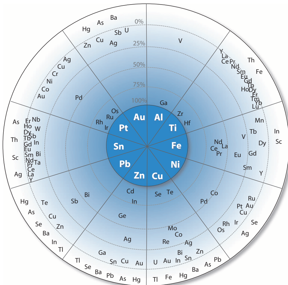
Fig. 2. The wheel of metal companionship. The principal host metals form the inner circle. Companion elements appear in the outer circle at distances proportional to the percentage of their primary production (from 100 to 0%) that originates with the host metal indicated. The companion elements in the white region of the outer circle are elements for which the percentage of their production that originates with the host metal indicated has not been determined. Data sources and assumptions for the assessment are given in the Supplementary Materials. Inspired by a diagram developed by (10).
