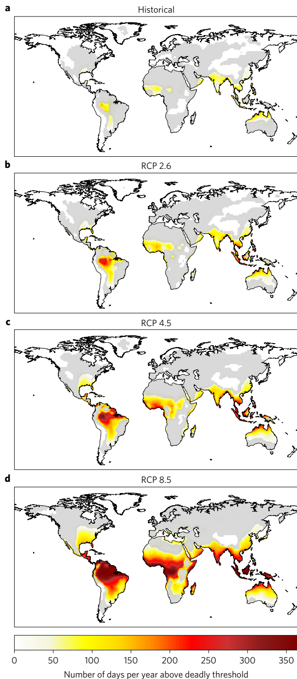
Figure 3 | Geographical distribution of deadly climatic conditions under different emission scenarios. a–d , Number of days per year exceeding the threshold of temperature and humidity beyond which climatic conditions become deadly (Fig. 1b), averaged between 1995 and 2005 (a, historical experiment), and between 2090 and 2100 under RCP 2.6 (b), RCP 4.5 (c) and RCP 8.5 (d). Results are based on multimodel medians. Grey areas indicate locations with high uncertainty (that is, the multimodel standard deviation was larger than the projected mean; coefficient of variance >1). The expected lower number of deadly days at higher latitudes (Fig. 4) may help explain the large variability among Earth System Models in the projected number of deadly days at higher latitudes 31 (for example, in the case for New York (illustrated in Fig. 4j) the one model projects nine deadly days by 2100; yet any other model projecting 18 days will double the variability). The uncertainty presented in this figure should be interpreted with that caution in mind.
