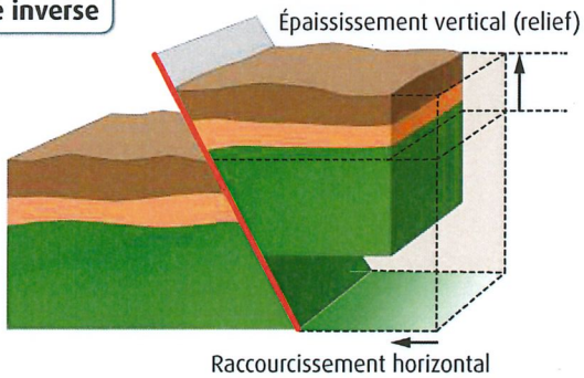
Faille inverse
