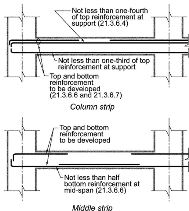
Fig. R21.3.6.3—Arrangement of reinforcement in slabs.
