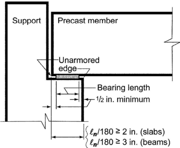
Fig. R16.6.2—Bearing length on support.
