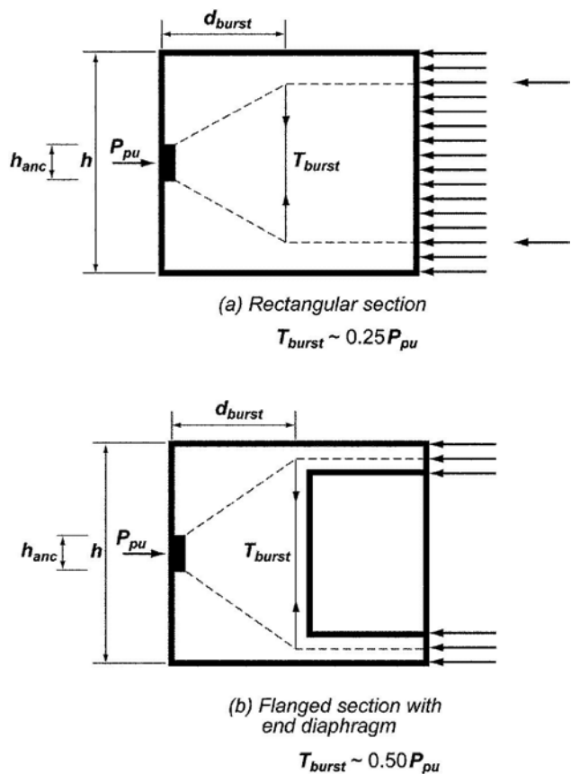
Fig. R18.13.3—Effect of cross section change.
