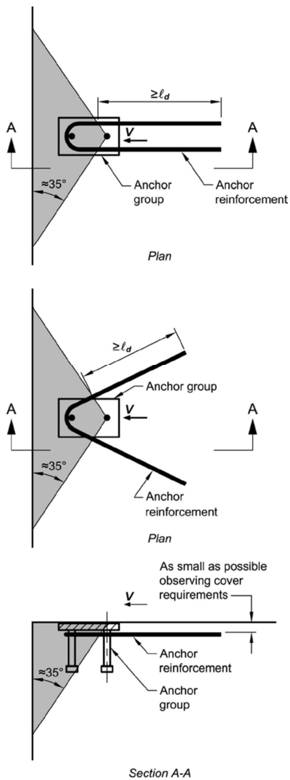
Fig. RD.6.2.9(a)—Hairpin anchor reinforcement for shear.
