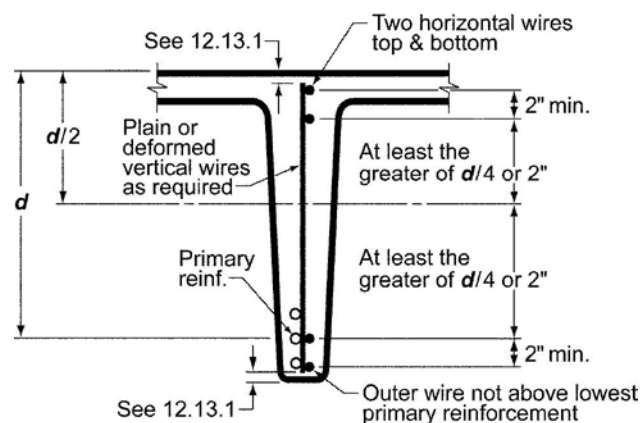
Fig. R12.13.2.4—Anchorage of single leg welded wire reinforcement shear reinforcement.
