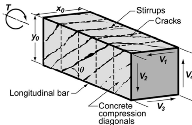
Fig. R11.5.3.6(a)—Space truss analogy.
