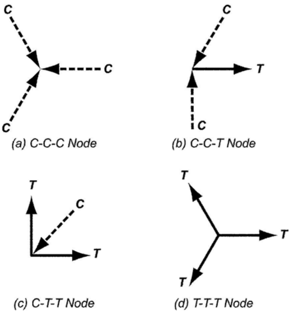
Fig. RA.1.7—Classification of nodes.
