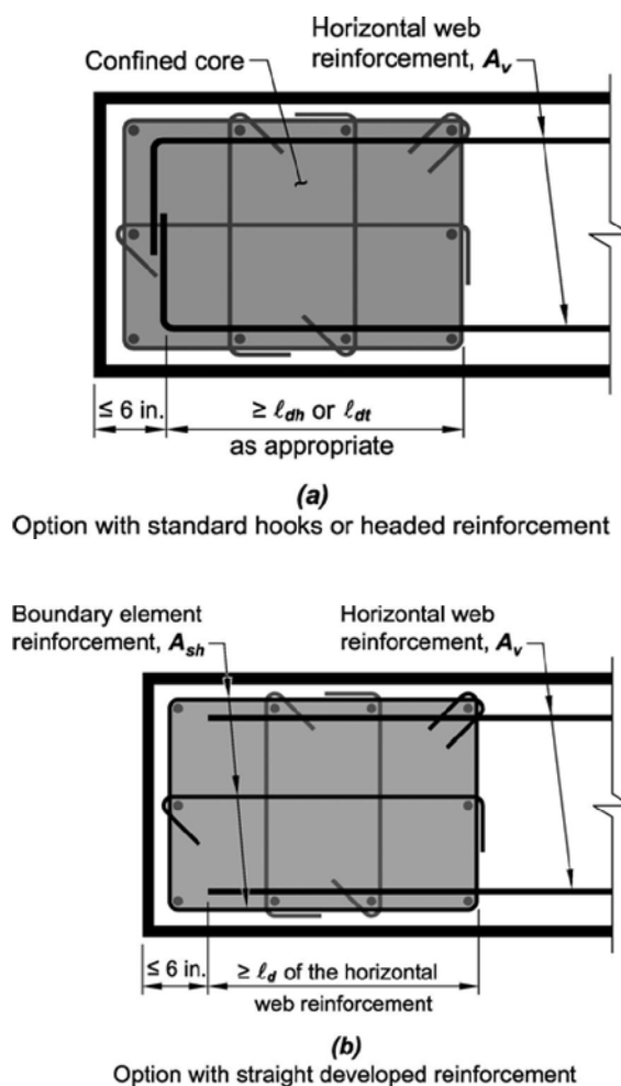
Fig. R.21.9.6.4—Development of wall horizontal reinforcement in confined boundary element.
