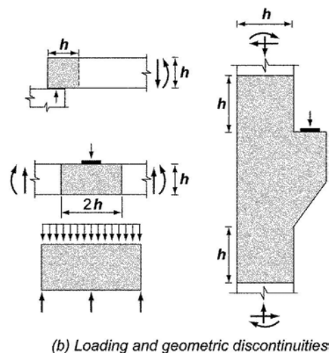
Fig. RA.1.1—D-regions and discontinuities.
