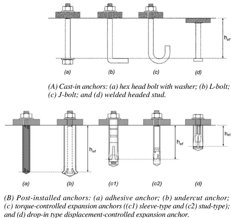
Fig. RD.1.1—Types of anchors.
