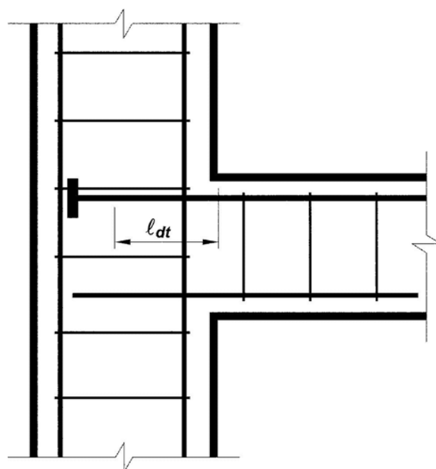
Fig. R12.6(b)—Headed deformed bar extended to far side of column core with anchorage length that exceeds \ell_{dt} .
