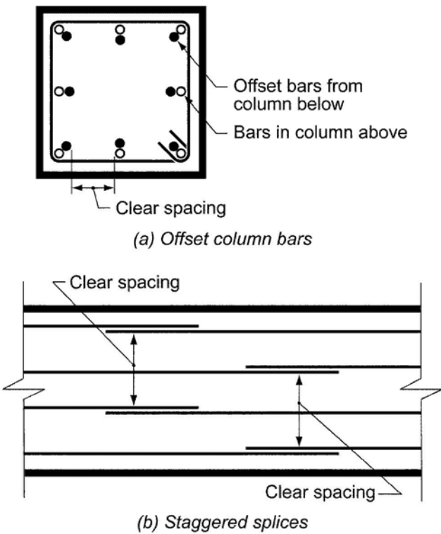
Fig. R12.15.1—Clear spacing of spliced bars.
