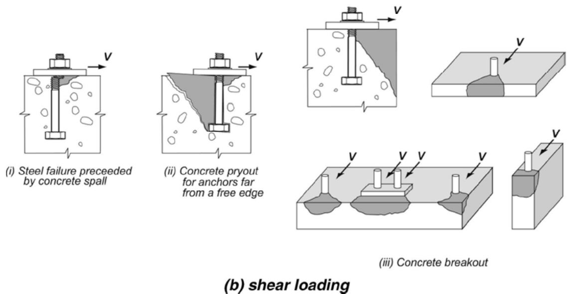
Fig. RD.4.1—Failure modes for anchors.
