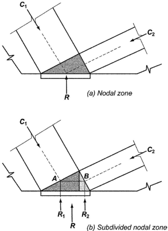
Fig. RA.1.6—Subdivision of nodal zone.
