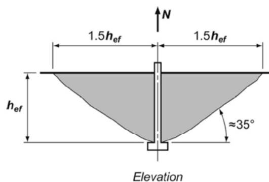
Fig. RD.4.2(a)—Breakout cone for tension.
