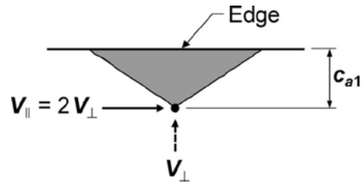
Fig. RD.6.2.1(c)—Shear force parallel to an edge.
