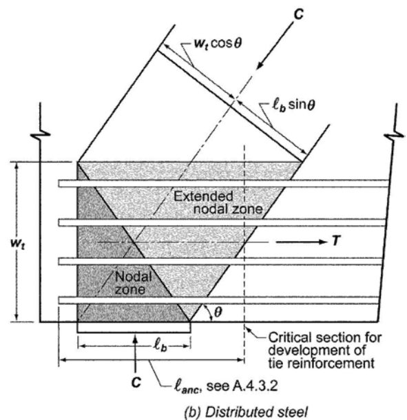
Fig. RA.1.5—Extended nodal zone showing the effect of the distribution of the force.
