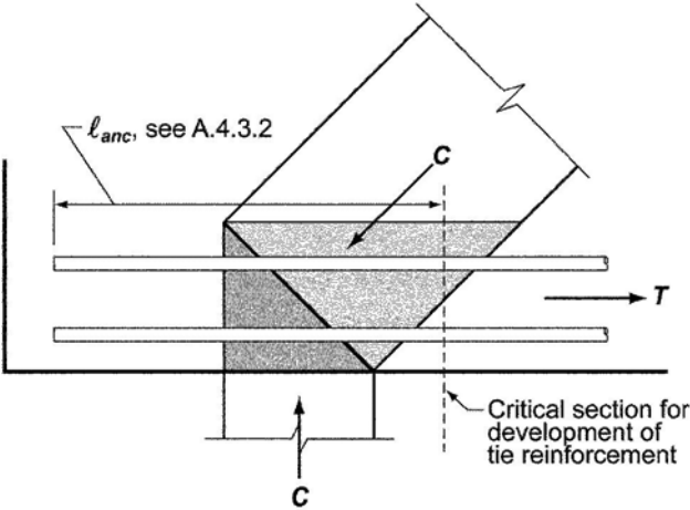
(b) Tension force anchored by a plate
