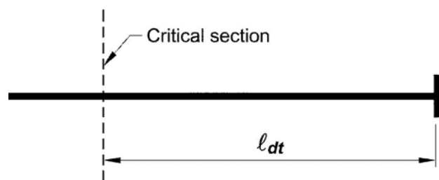
Fig. R12.6(a)—Development of headed deformed bars.
