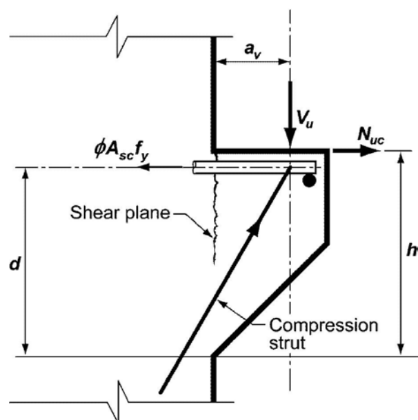
Fig. R11.8.1—Structural action of a corbel.
