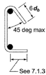
(a) single-leg stirrup or bar
