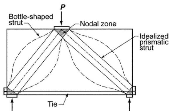
Fig. RA.1.3—Description of strut-and-tie model.
