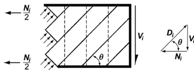
Fig. R11.5.3.7—Resolution of shear force V_i into diagonal compression force D_i and axial tension force N_i in one wall of the tube.
