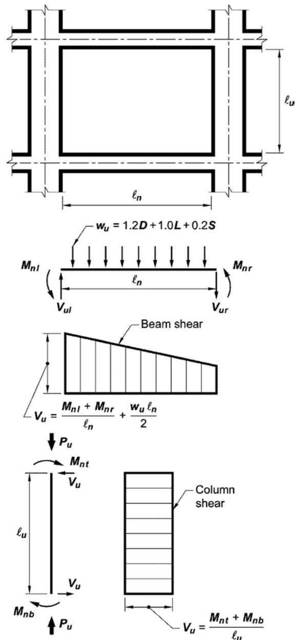
Fig. R21.3.3—Design shears for intermediate moment frames.
