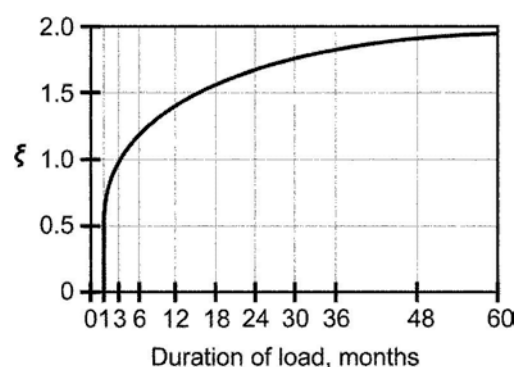
Fig. R9.5.2.5—Multipliers for long-term deflections.
