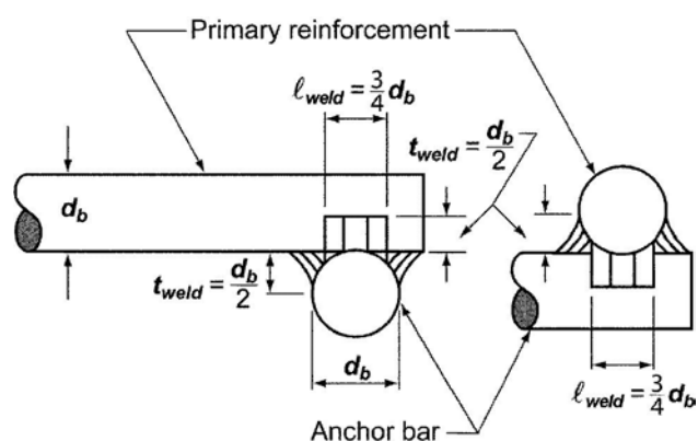
Fig. R11.8.6—Weld details used in tests of Reference 11.56.
