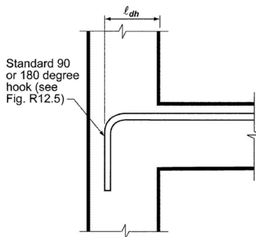
(a) Anchorage into exterior column
