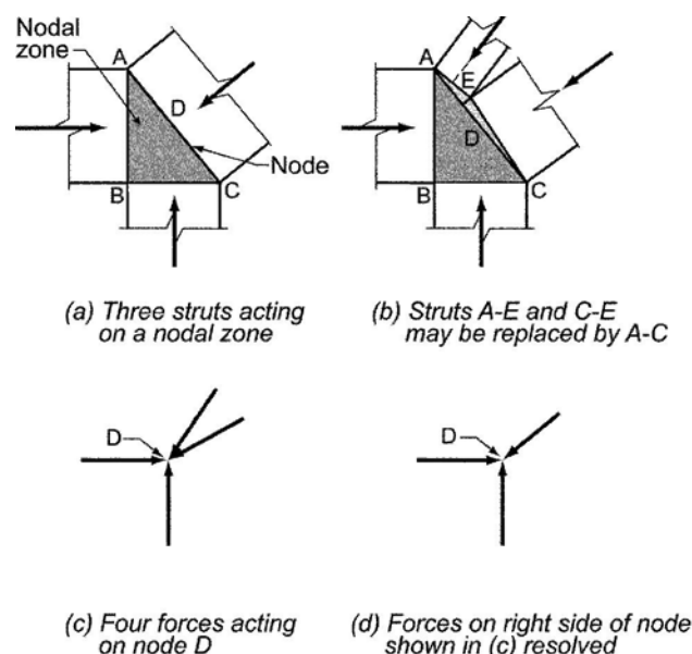
Fig. RA.2.3—Resolution of forces on a nodal zone.
