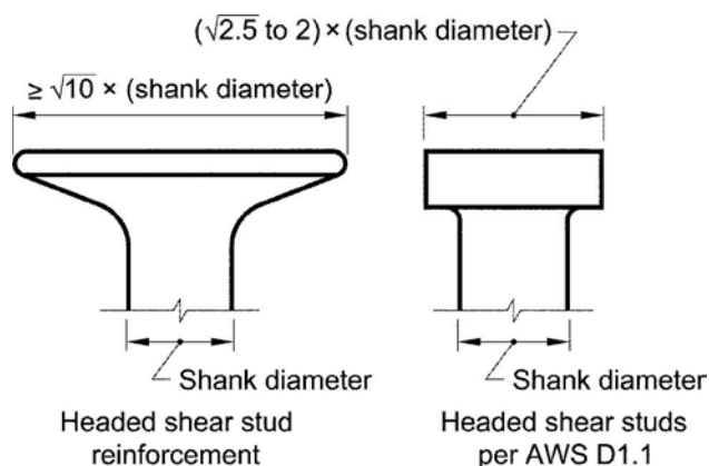
Fig. R3.5.5—Configurations of stud heads.
