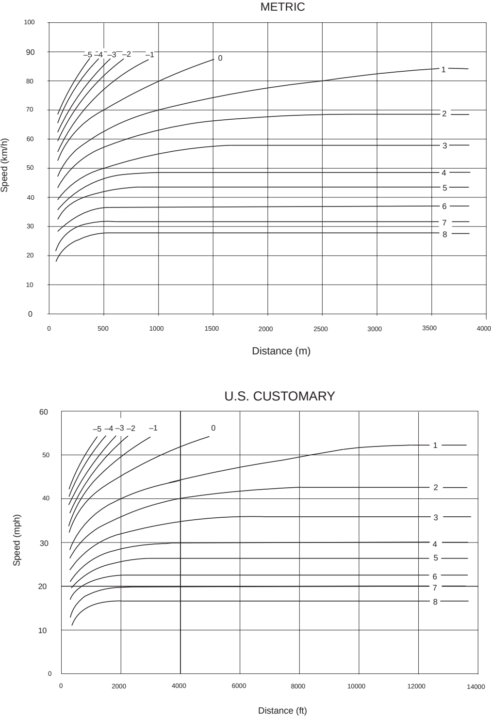
Figure 3-25. Speed-Distance Curves for Acceleration of a Typical Heavy Truck of 120 kg/kW [200 lb/hp] on Upgrades and Downgrades
