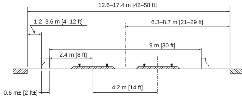
Typical Roadway Section – A –
