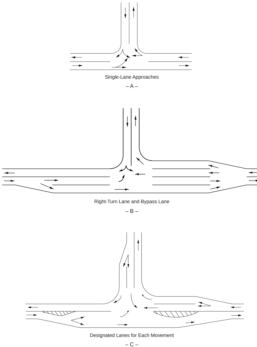
Figure 9-4. Three-Leg Intersections
