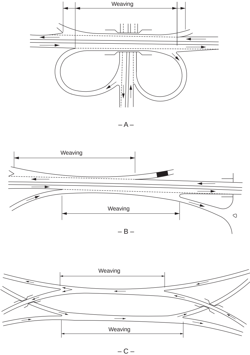
Figure 2-30. Weaving Sections
