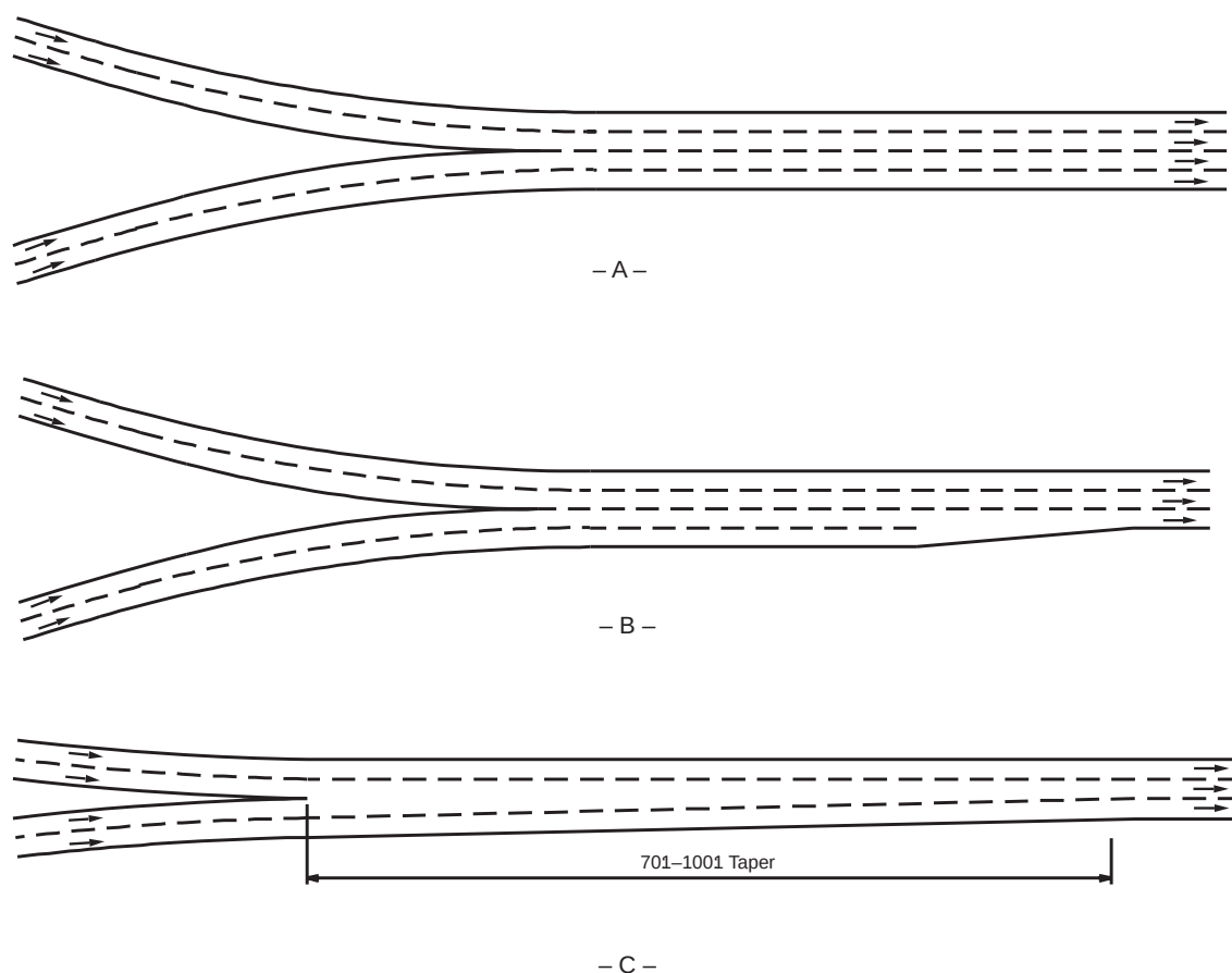
Figure 10-76. Branch Connections
