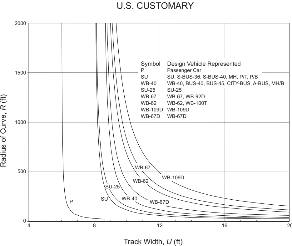
Figure 3-17. Track Width for Widening of Traveled Way on Curves
