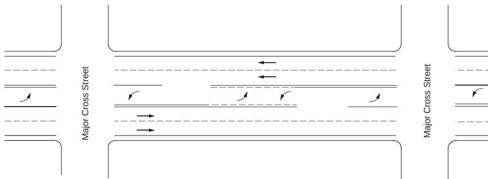
Typical Multilane Highway with Flush or Transversable Lane at Midblock
