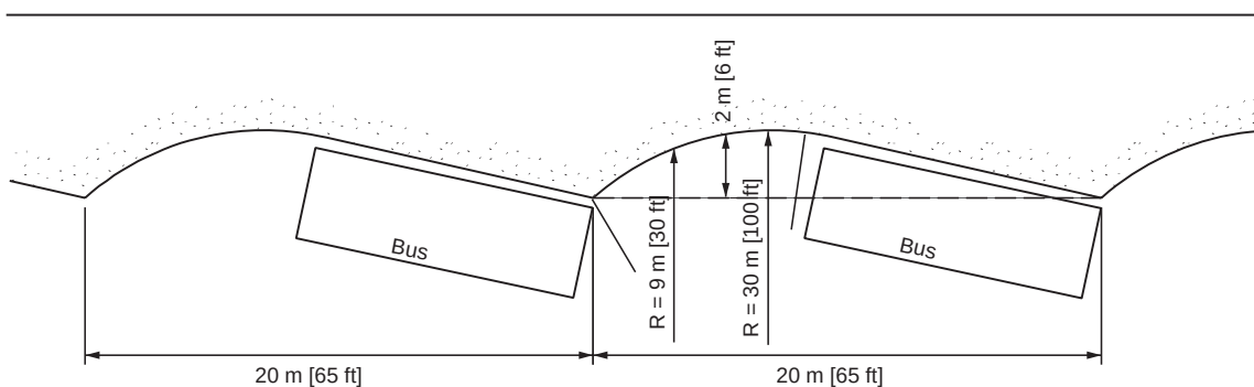
Figure 4-24. Sawtooth Bus Loading Area
