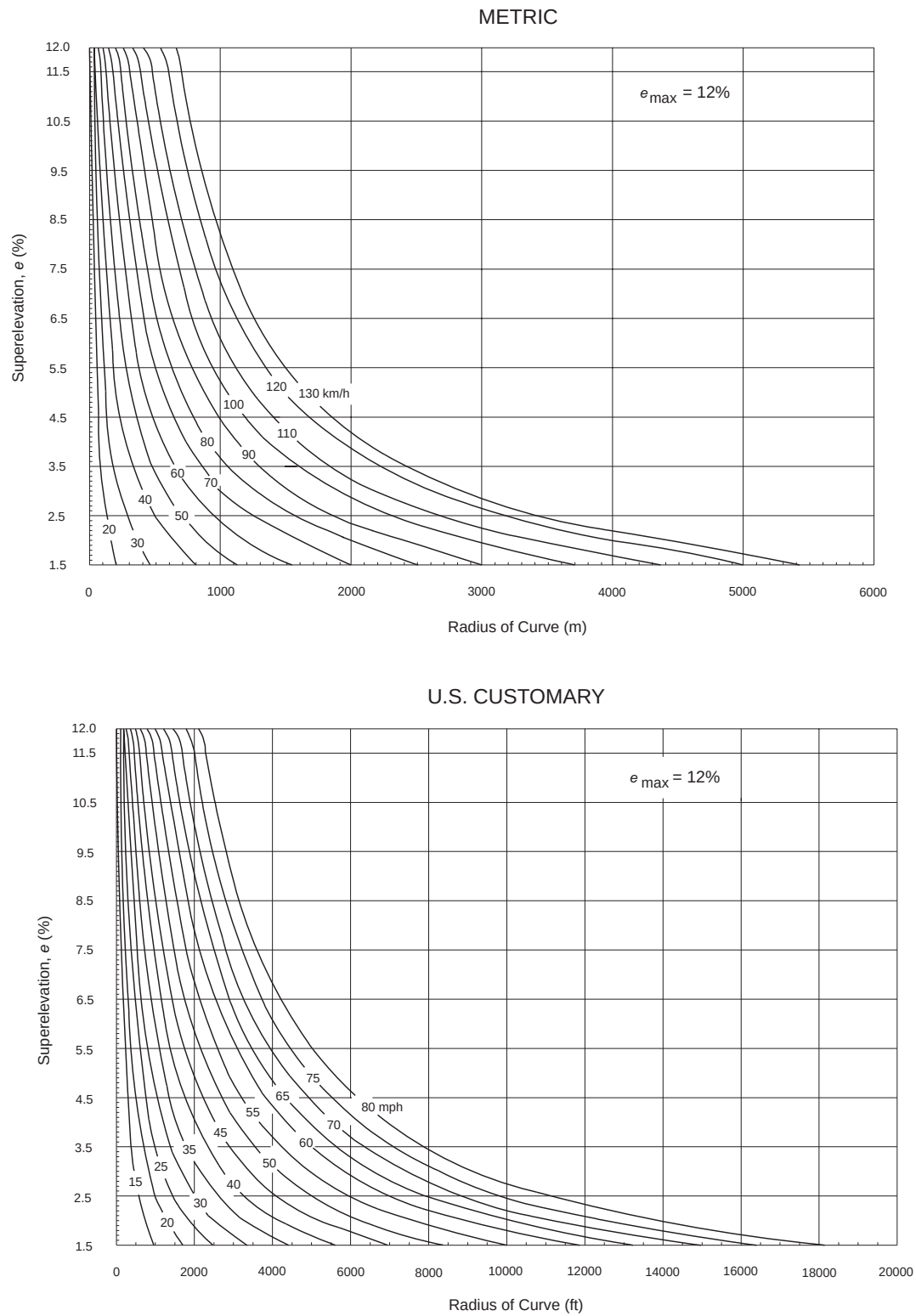
Figure 3-13. Design Superelevation Rates for Maximum Superelevation Rate of 12 Percent
