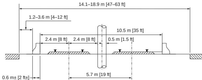
At Underpass with One Pier – B –
