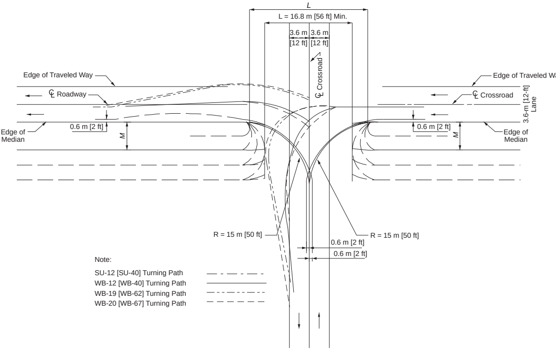
Figure 9-56. Minimum Design of Median Openings (SU-9 [SU-30] Design Vehicle, Control Radius of 15 m [50 ft])
