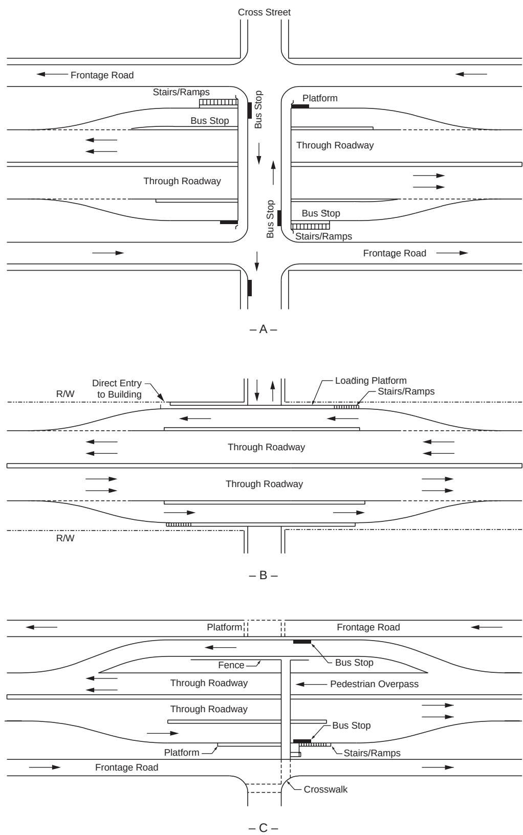
Figure 8-24. Bus Stops at Freeway Level
