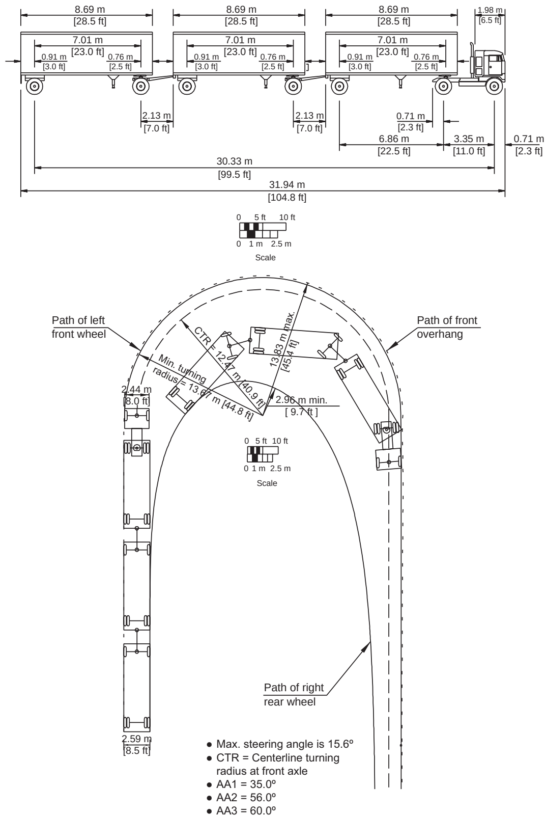
Figure 2-18. Minimum Turning Path for Triple-Trailer Combination (WB-30T [WB-100T]) Design Vehicle
