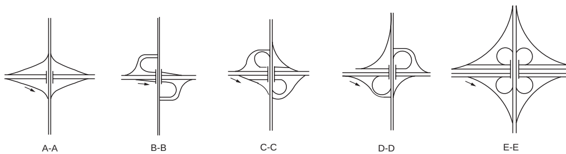
Uniform Patterns of Exits
