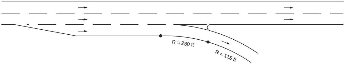
Compound Curve, Radii = 230 ft and 115 ft – B –
