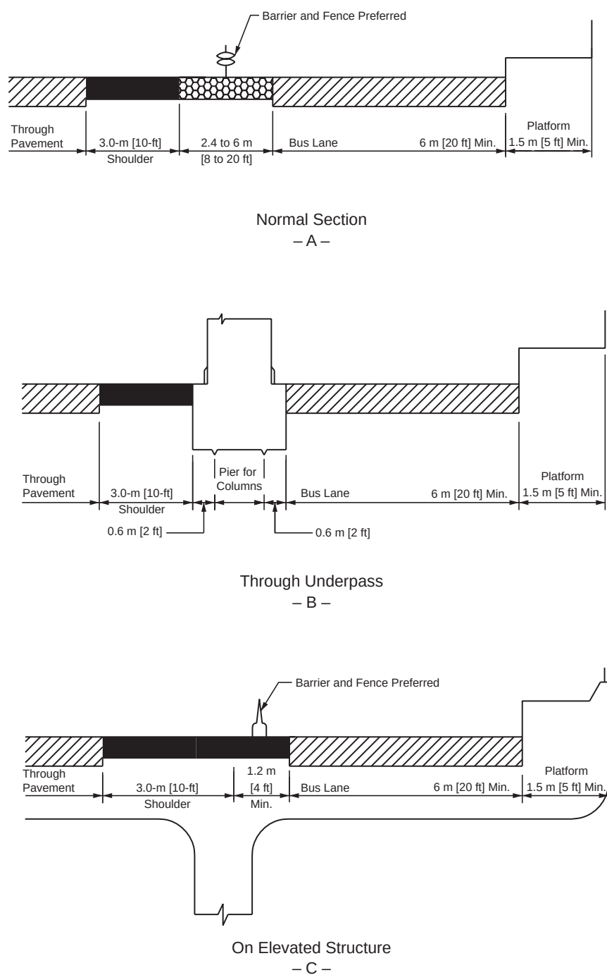
Figure 4-22. Bus Turnouts
