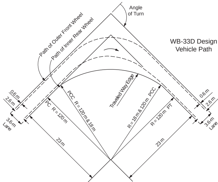
WB-33D Double Trailer Combination, Centered Compound Curve, 120 m – 18 m – 120 m Radii, Offset 5 m
