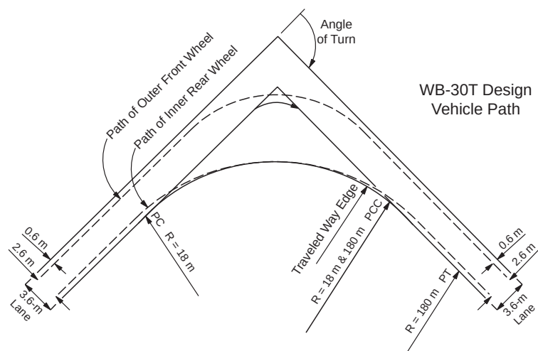
WB-30T Triple Trailer Combination, Compound Curve, 18-m and 180-m Radii
