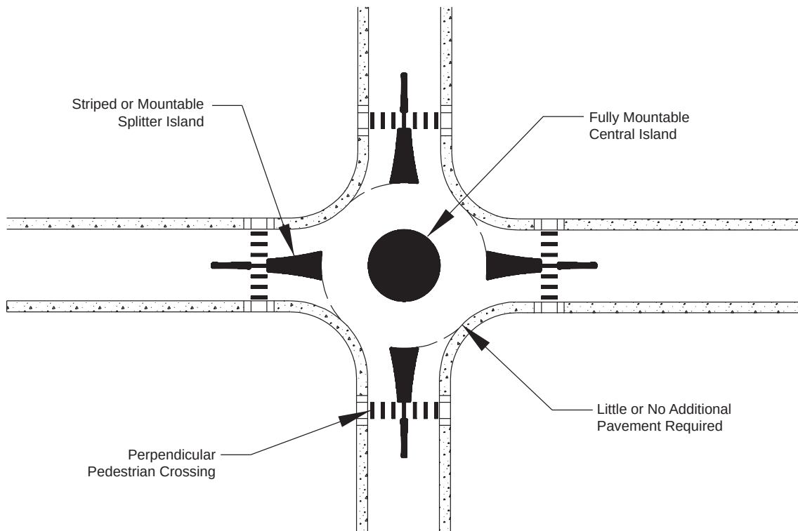
Figure 9-11. Typical Mini-Roundabout
