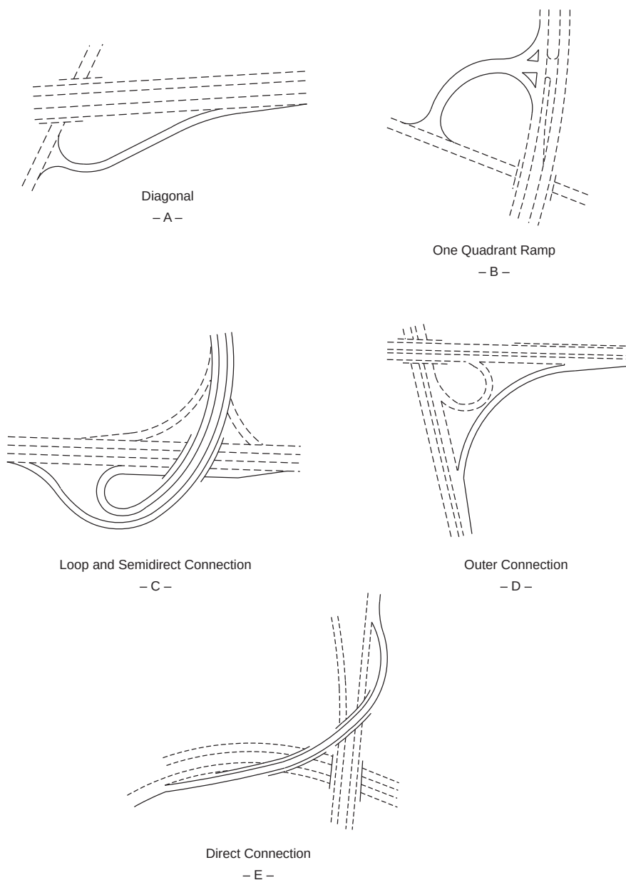
Figure 10-58. General Types of Ramps
