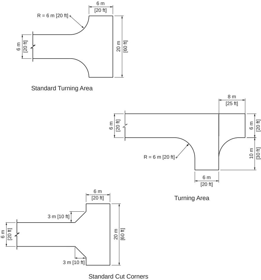
Figure 5-2. Alley Turnarounds
