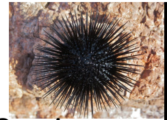
Oursin
